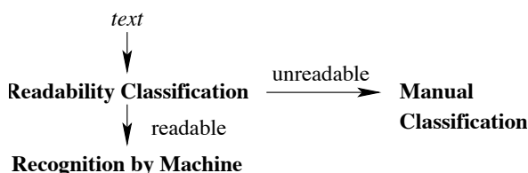
Figure 1: Readability Classification
