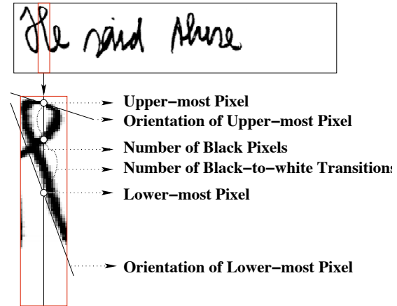
Figure 3: Local Features Extracted by the Sliding Window
